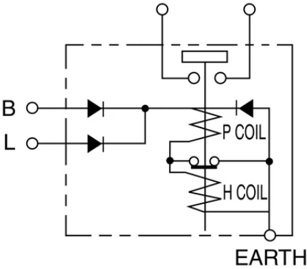
MAIN TERMINALS
