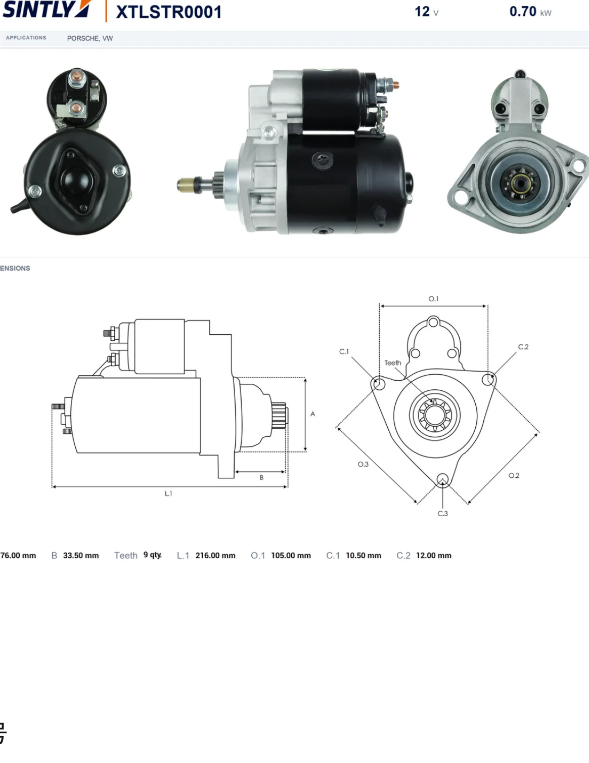
A 76.00 mm B 33.50 mm Teeth 9 qty L.1 216.00 mm O.1 105.00 mm C.1 10.50 mm C.2 12.00 mm
